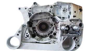
Crankcase Left Part NO.GT73-CE00-004
